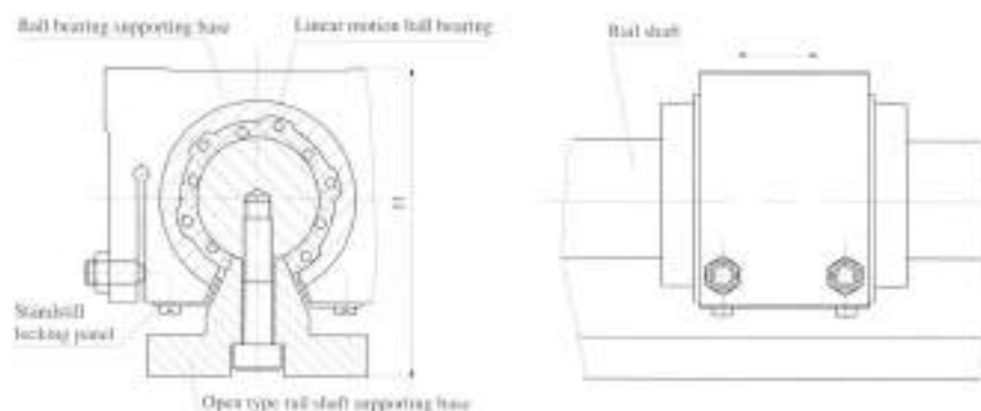
Fig. 1 GTA open-type linear motion bushing
