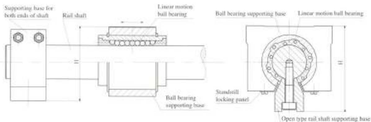
Fig. 2 GTB close-type linear motion bushing
