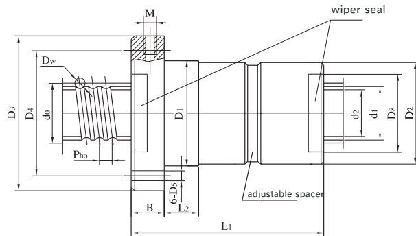
Mounting &amp; connecting dimension
